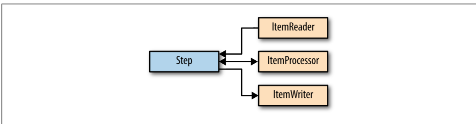
Figure 13-8. Spring Batch step components
